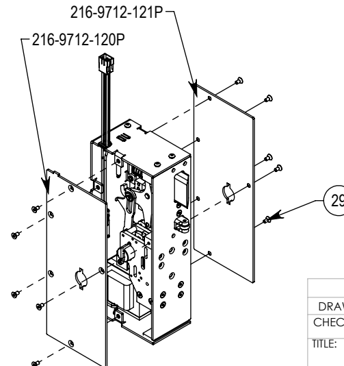
Right Hand Keyed Both Sides
