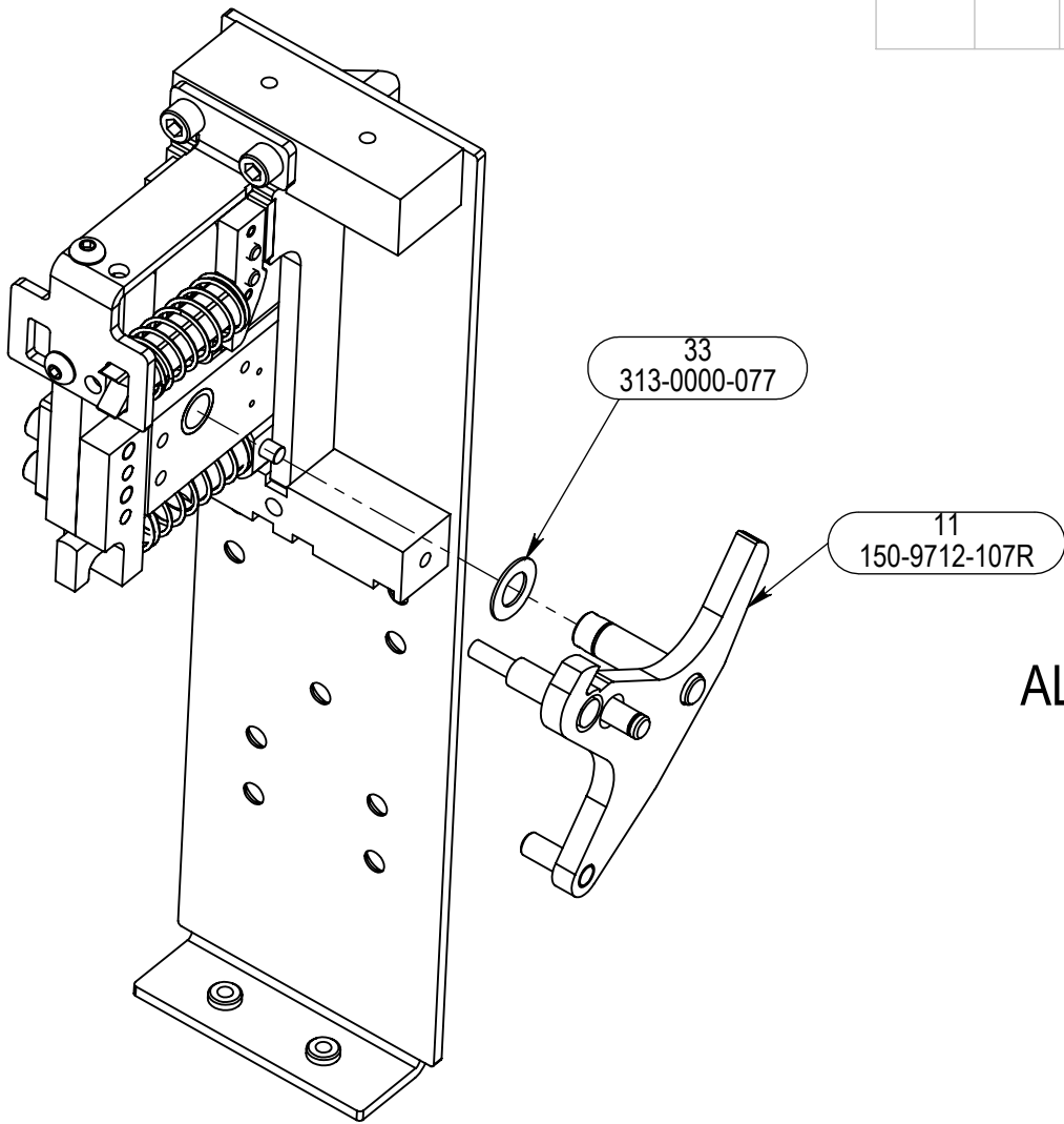
146-9712-500R Right Handed
