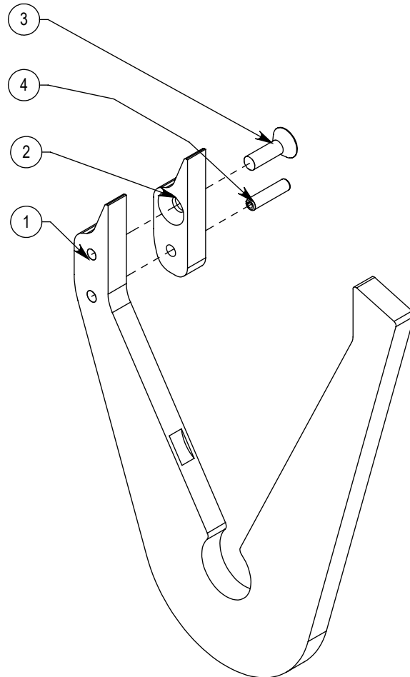
146-9712-301R RLB Pawl Assembly Right
