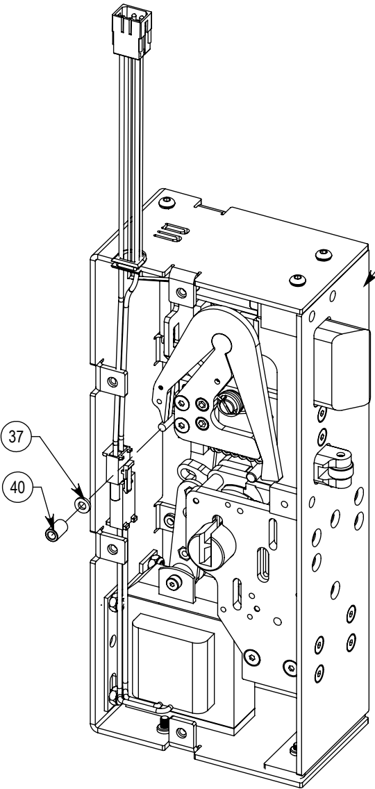
Left Hand Lock with RLB
