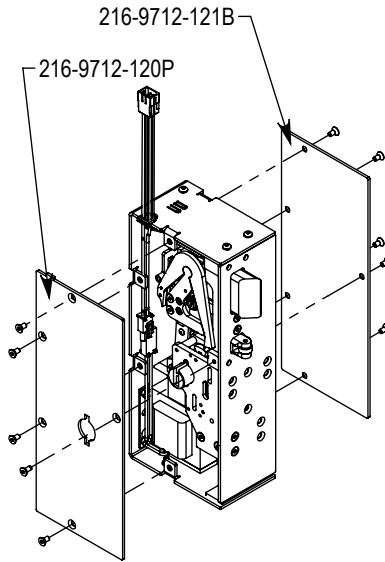
Left Hand Keyed Hinge Side
